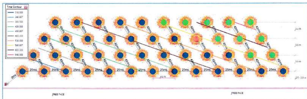
Fig. 7.14: Diagonal sequence of rock movement and time contour obtained from the recommended firing patterns in Figures 7.13
